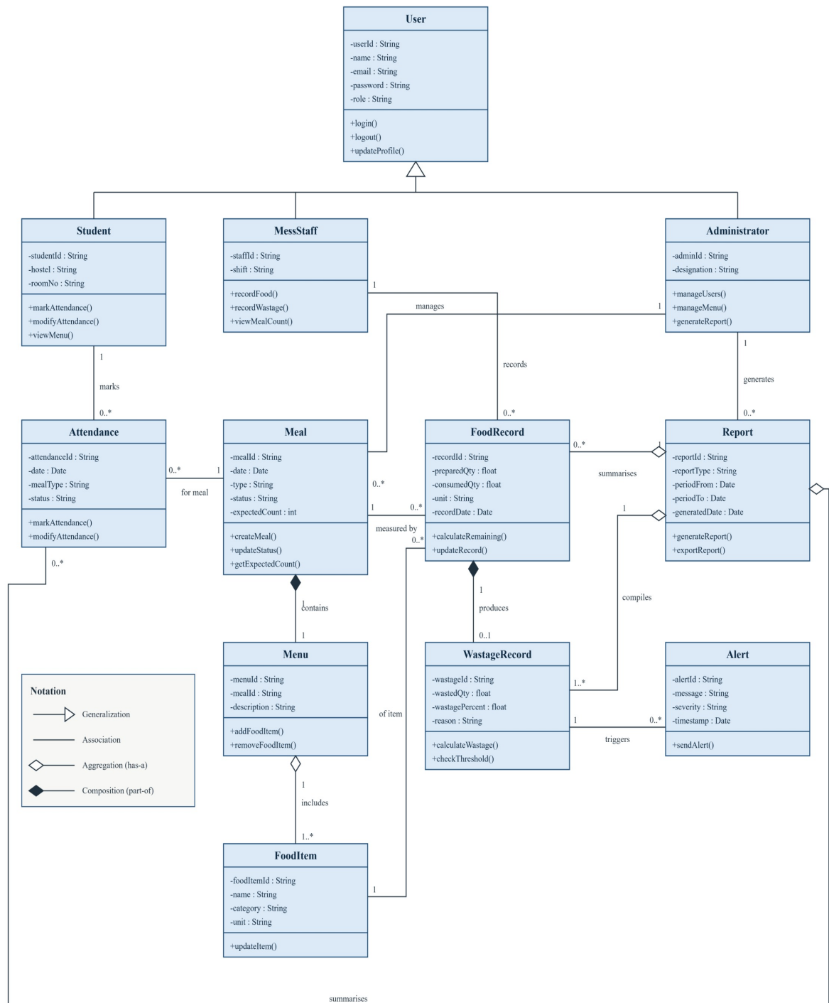
Figure 8.6: Class Diagram
