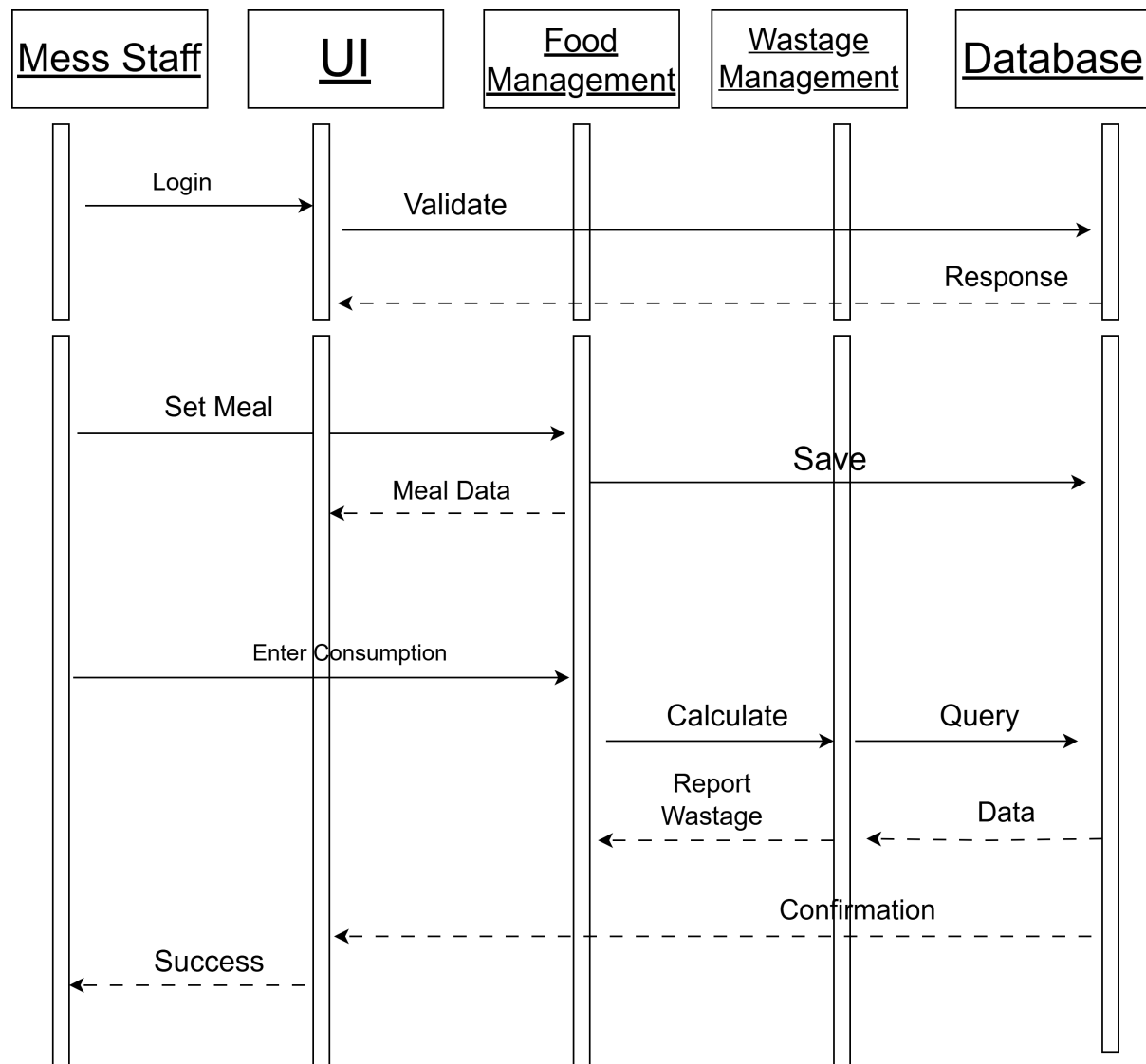
Figure 9.3: Sequence Diagram for Recording Food Wastage
